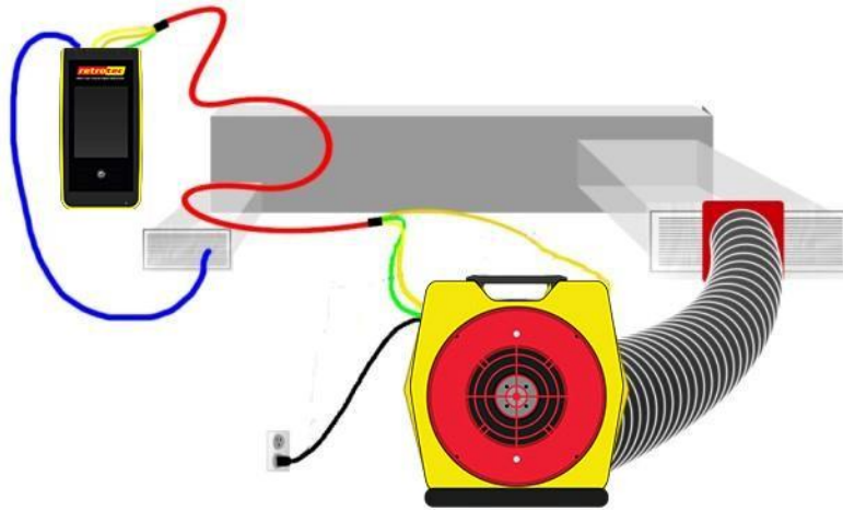
Figure 9: DuctTester setup, including tubing locations and necessary connections.
