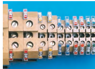
Terminal Blocks
