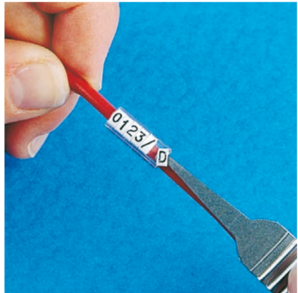
Step 4 Marking elements can be added or removed as required with removal hook
